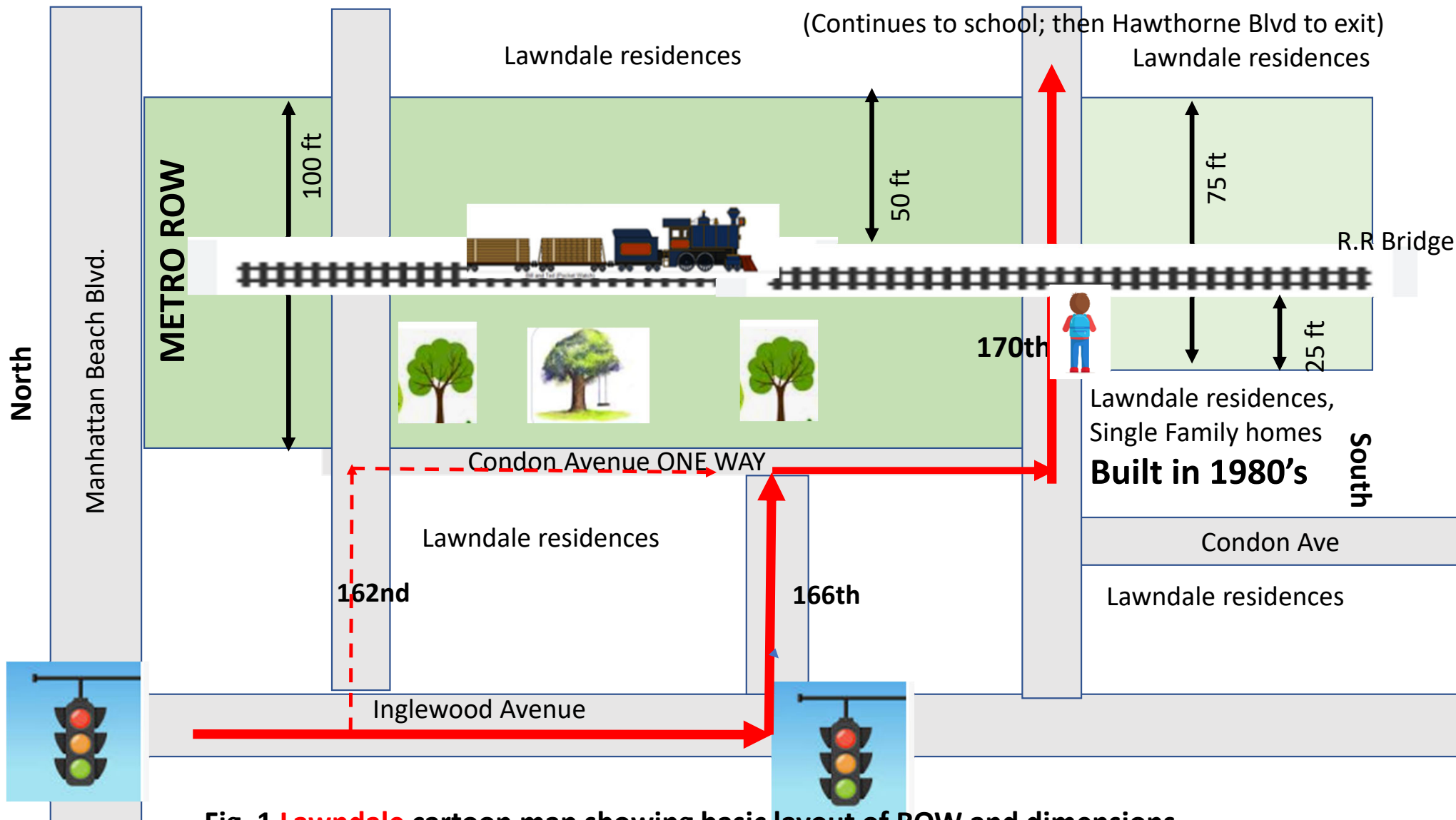
Fig. 1 Lawndale cartoon map showing basic layout of ROW and dimensions
