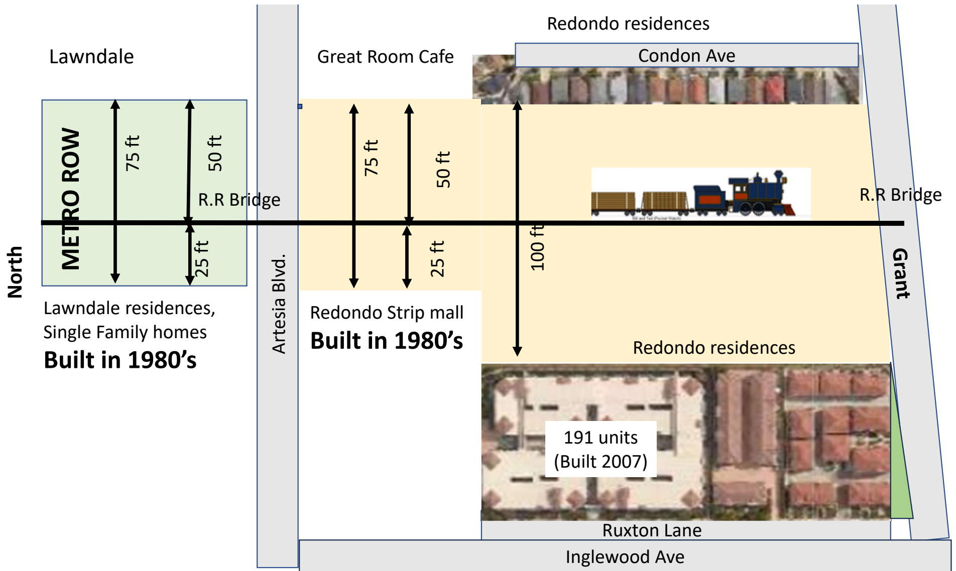
Fig. 2. Redondo ROW layout south of Artesia to Grant, showing dimensions
